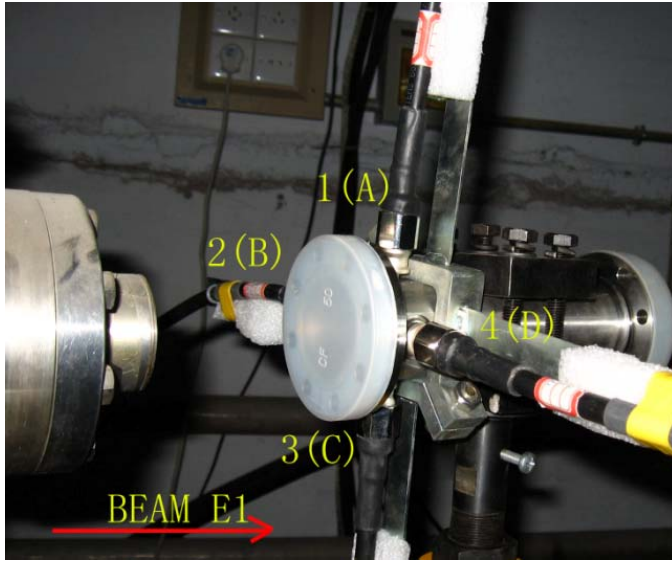
Fig.1 BPM at E1 line
