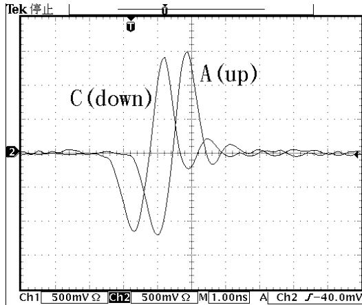
Fig3. Typical pickup signals of BPM02 at the end of 40m coaxial cables
