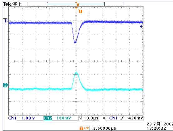
Fig3. Typical pickup signals of BPM02 at the end of 40m coaxial cables
